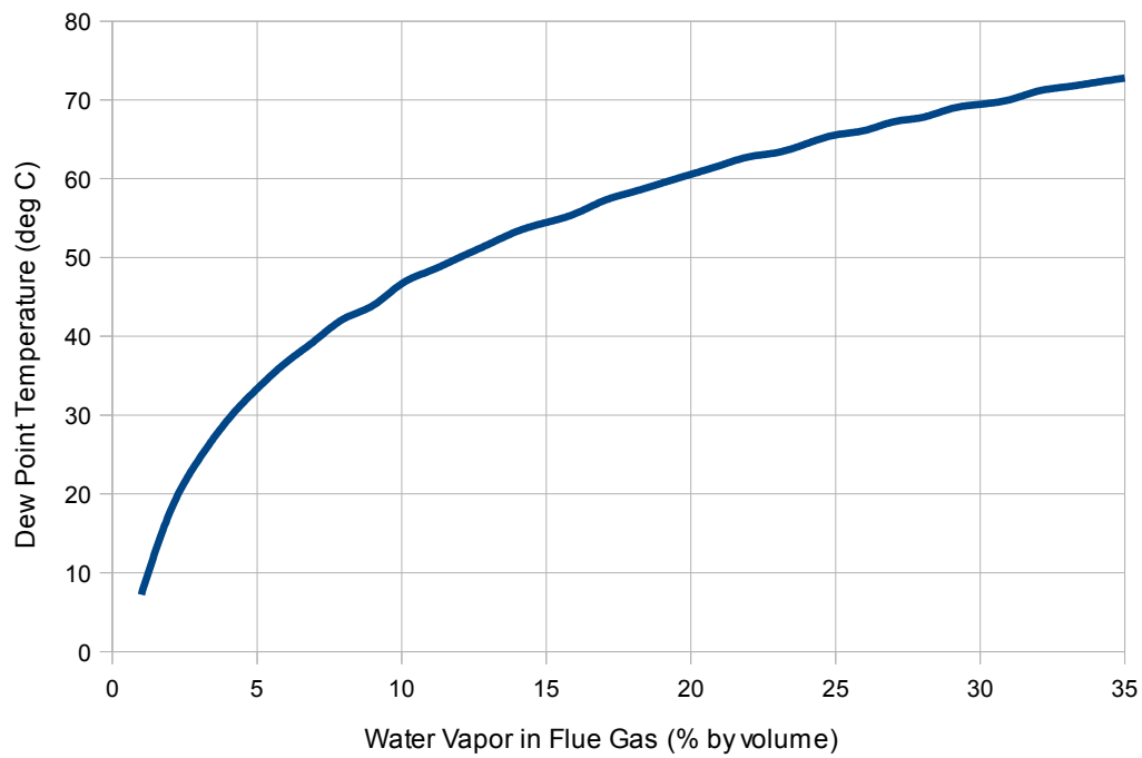
Dew Point Temperature of Flue Gases
