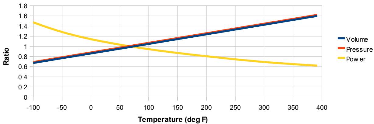
Fans - Temperature Flow, Pressure and Power Consumption
